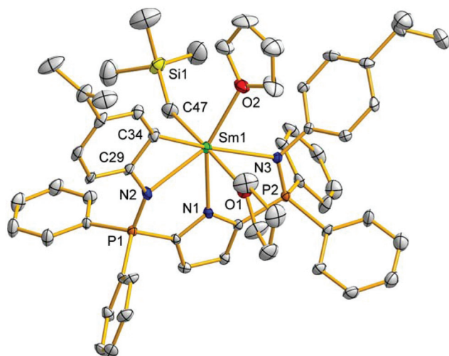
Fig. 2 Thermal displacement plot (20% probability) of complex 2 with hydrogen atoms and minor disordered components omitted for clarity. Selected bond distances (Å) and angles ( ^\circ ): P1–N2 = 1.571(6), P2–N3 = 1.593(6), Sm1–N1 = 2.454(5), Sm1–N2 = 2.436(6), Sm1–N3 = 2.582(6), Sm1–C34 = 2.551(7), Sm1–C47 = 2.47(1), Sm1–O1 = 2.588(6), Sm1–O2 = 2.480(6); C1–P1–N2 = 102.3(3), C4–P2–N3 = 105.6(3), C47–Sm1–O1 = 177.1(3), N1–Sm1–C34 = 122.7(2).
