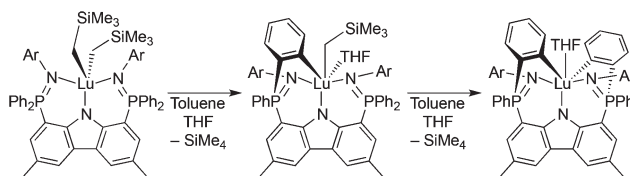
Scheme 1 Cyclometalative behaviour of a carbazole-based bisphosphinimine lutetium complex.
