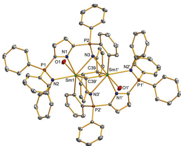
Fig. 3 Thermal displacement plot (30% probability) of complex 3 with hydrogen atoms, benzene solvent molecules, THF backbones, Pipp 1 Pr groups, and minor disordered components omitted for clarity. Symmetry code ' = 2 – x, –y, –z. Selected bond distances (Å) and angles (°): P1–N2 = 1.600(2), P2–N3 = 1.609(1), Sm1–N1 = 2.477(2), Sm1–N2 = 2.530(2), Sm1–N3 = 2.616(2), Sm1–C39 = 2.638(2), Sm1–C27' = 2.597(2), Sm1–O1 = 2.575(2), Sm1...Sm1' = 3.3655(6); P2–N3–C38 = 136.7(1), N3–P2–C26 = 109.0(1).
