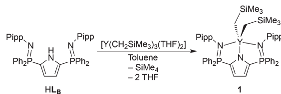
Scheme 2 Formation of pyrrole-based bisphosphinimine yttrium complex 1 .
