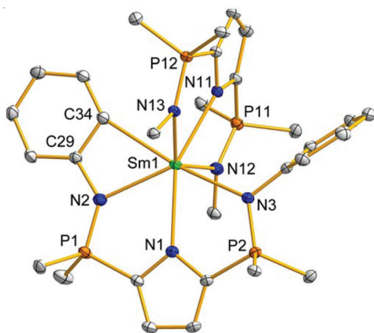
Fig. 4 Thermal displacement plot (30% probability) of complex 4 with hydrogen atoms, P -phenyl rings (except ipso carbons), N -aryl rings (except ipso carbons) on the non-cyclometalated ligand and isopropyl substituents on the cyclometalated ligand omitted for clarity. Selected bond distances (Å) and angles (°): P1–N2 = 1.577(3), P2–N3 = 1.597(3), Sm1–N1 = 2.509(3), Sm1–N2 = 2.471(3), Sm1–N3 = 2.615(3), Sm1–C34 = 2.603(4), Sm1–N11 = 2.466(2), Sm1–N12 = 2.469(2), Sm1–N13 = 2.472(3); N12–Sm1–N13 = 136.21(9).
