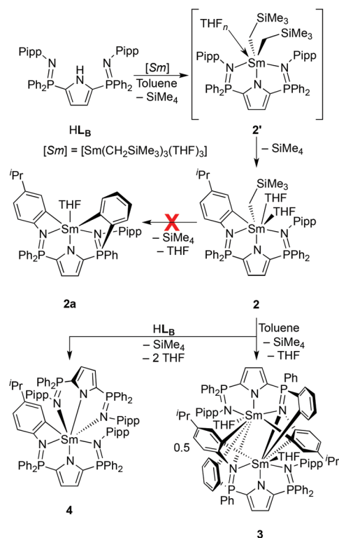
Scheme 3 Synthesis of bisphosphinimine-ligated samarium complexes.
