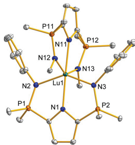
Fig. 5 Thermal displacement plot (30% probability) of the cation of complex 5 with hydrogen atoms, non- ipso carbons of the P -phenyl rings, non- ipso carbons of the N12 and N13 N -aryl rings, isopropyl groups of the N2 and N3 N -aryl rings and minor disordered components omitted for clarity. Selected bond distances (Å) and angles (°): P1–N2 = 1.634(2), P2–N3 = 1.637(2), P11–N12 = 1.642(2), P12–N13 = 1.637(2), Lu1–N1 = 2.340(2), Lu1–N2 = 2.324(2), Lu1–N3 = 2.326(2), Lu1–N11 = 2.338(2), Lu1–N12 = 2.326(2), Lu1–N13 = 2.352(2); N1–Lu1–N11 = 178.22(7), N2–Lu1–N3 = 143.90(7), N12–Lu1–N13 = 143.60(7).
