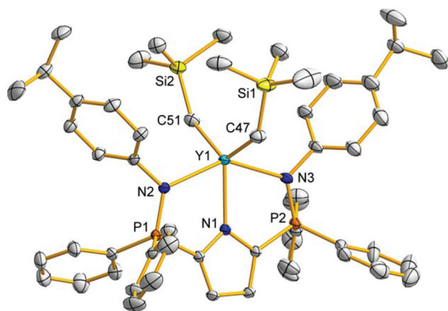
Fig. 1 Thermal displacement plot (30% probability) of complex 1 with hydrogen atoms and minor disordered components omitted for clarity. Selected bond distances (Å) and angles (°): P1–N2 = 1.606(2), P2–N3 = 1.609(2), Y1–N1 = 2.345(2), Y1–N2 = 2.374(2), Y1–N3 = 2.410(2), Y1–C47 = 2.412(3), Y1–C51 = 2.394(3); C1–P1–N2 = 103.3(1), C4–P2–N3 = 104.2(1), C47–Y1–C51 = 127.3(1), N2–Y1–N3 = 141.96(7).
